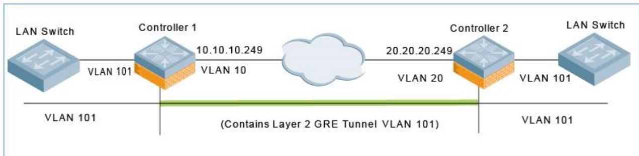
Figure 14 Layer-2 GRE Tunnel
