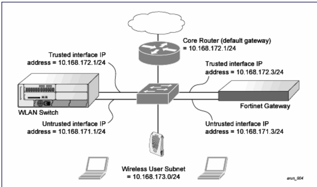
Figure 126 Example Route-Mode Topology
