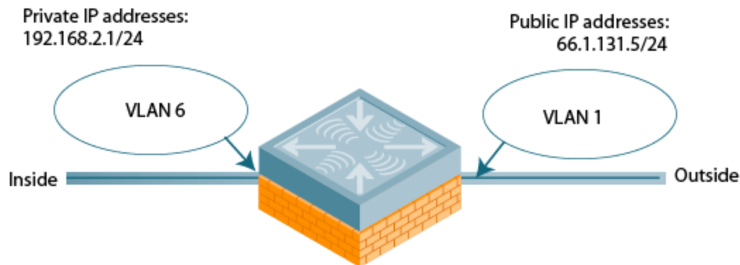
Figure 12 Example: Source NAT using the IP Address of Managed Device
