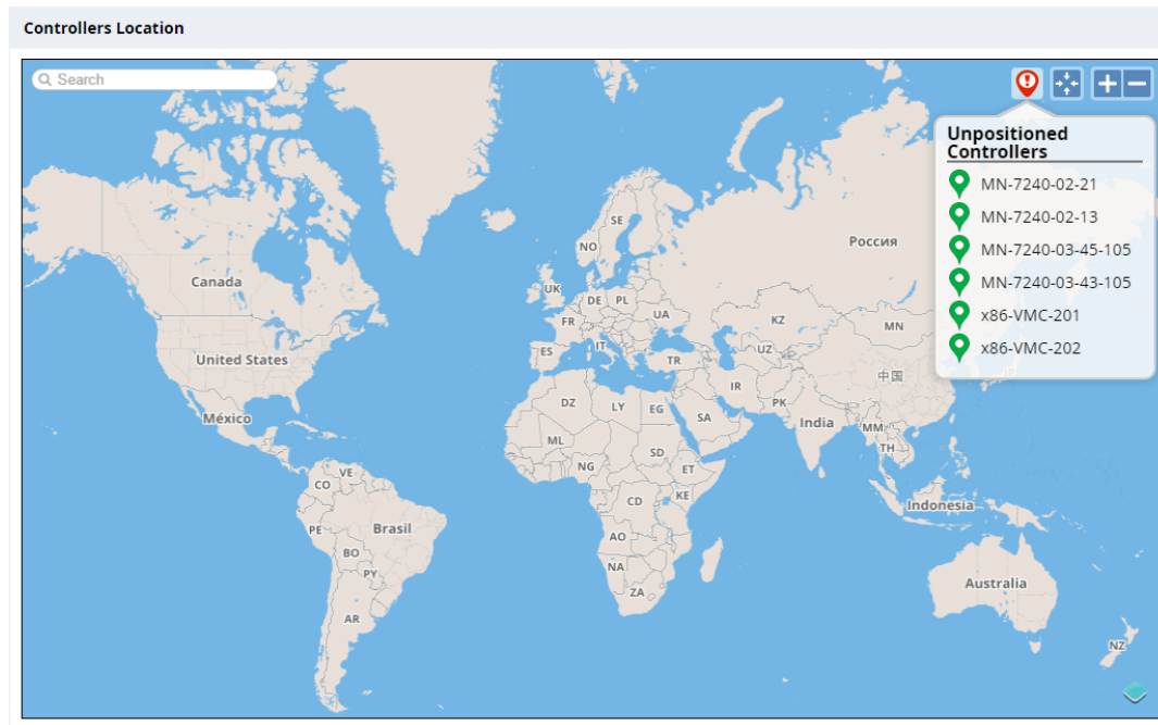
Figure 56 Network Page
