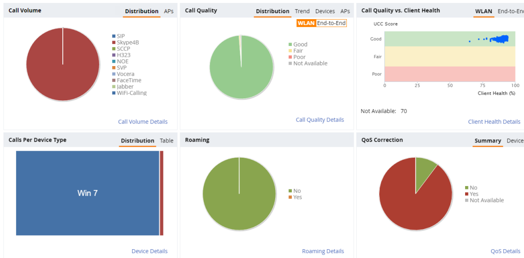
Figure 113 UCC Dashboard
