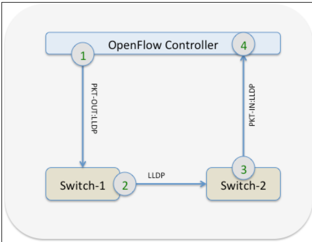
Figure 109 Topology Discovery
