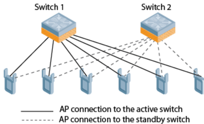
Figure 42 1:1 Active/Standby Deployment
