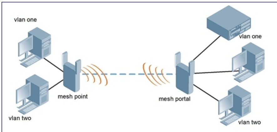
Figure 38 Sample Point-to-Point Deployment
