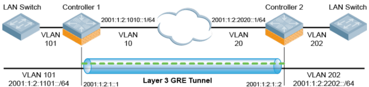
Figure 16 IPv6 Layer-3 GRE Tunnel
