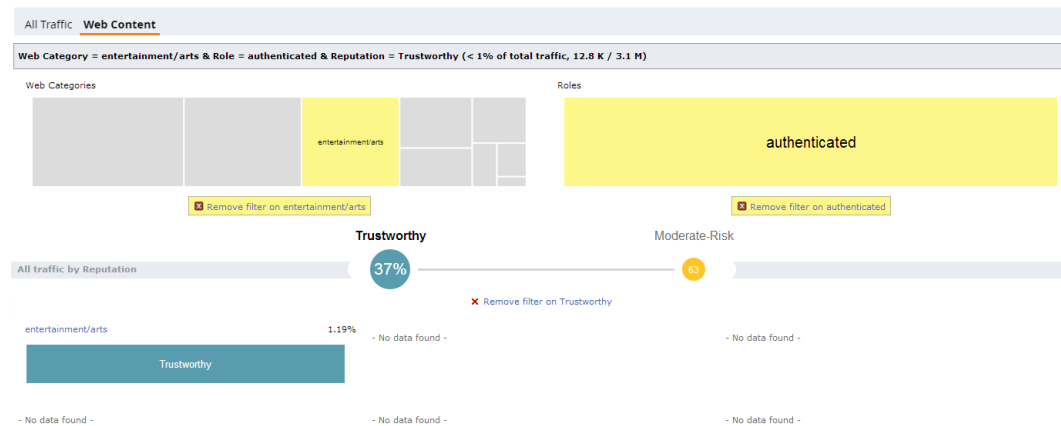
Figure 77 Multiple Filters
