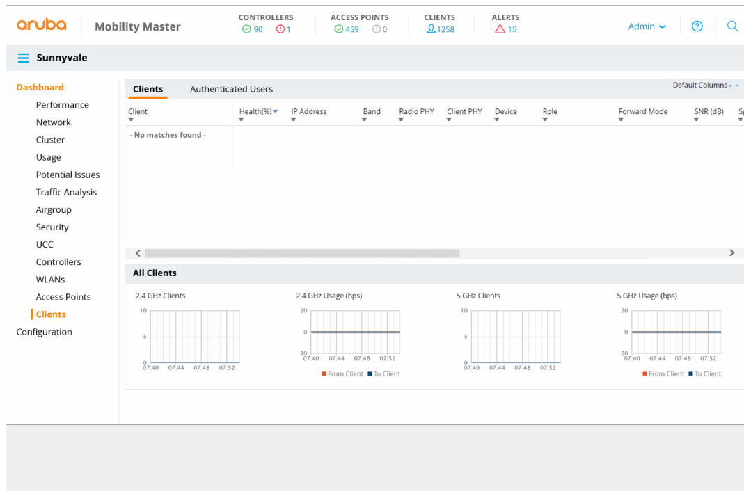
Figure 90 Clients Page
