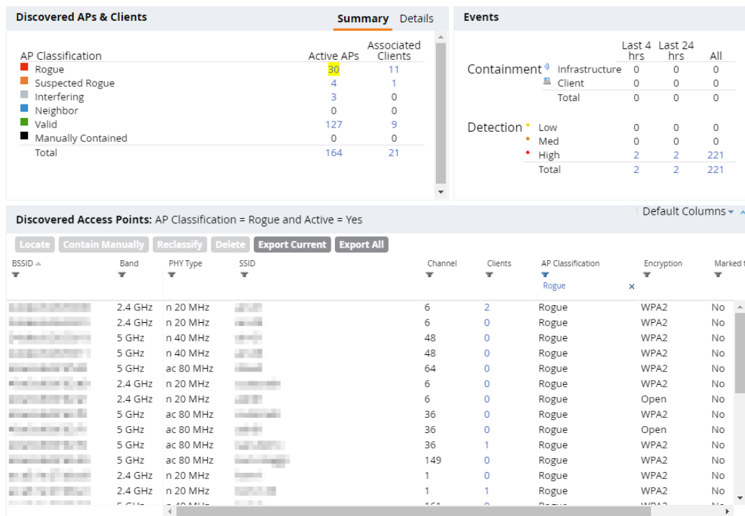
Figure 82 Security Page
