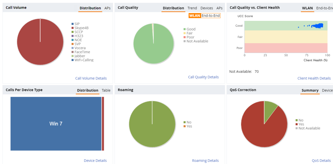
Figure 83 UCC Dashboard
