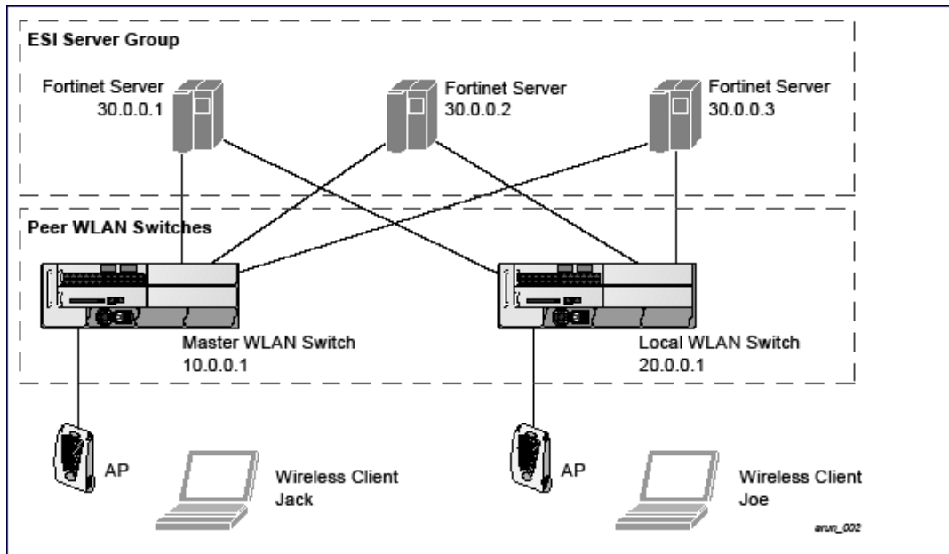
Figure 125 Peer managed device
