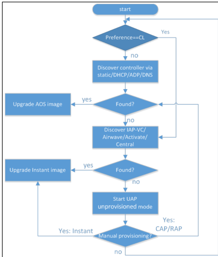
Figure 34 AP Discovery Logic
