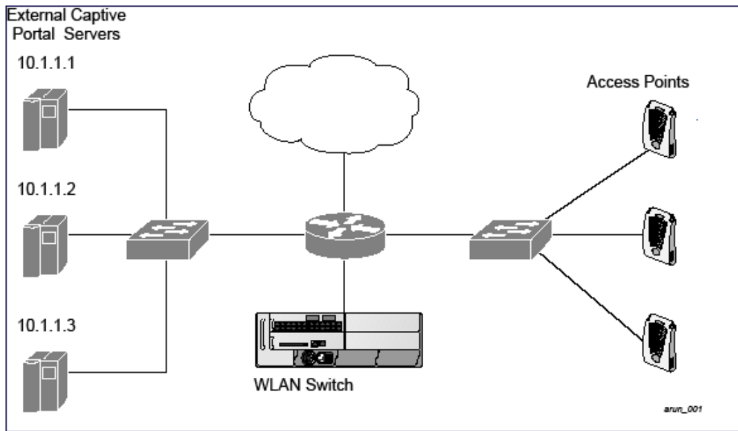
Figure 127 Example NAT-Mode Topology
