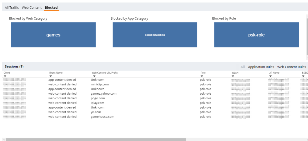
Figure 78 Blocked Tab
