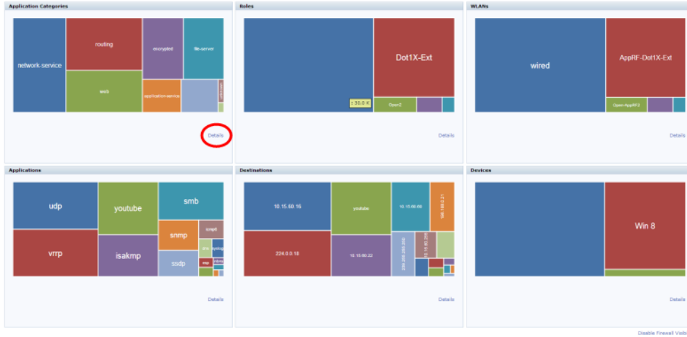
Figure 66 Details
