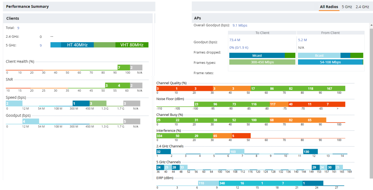
Figure 55 Performance Page
