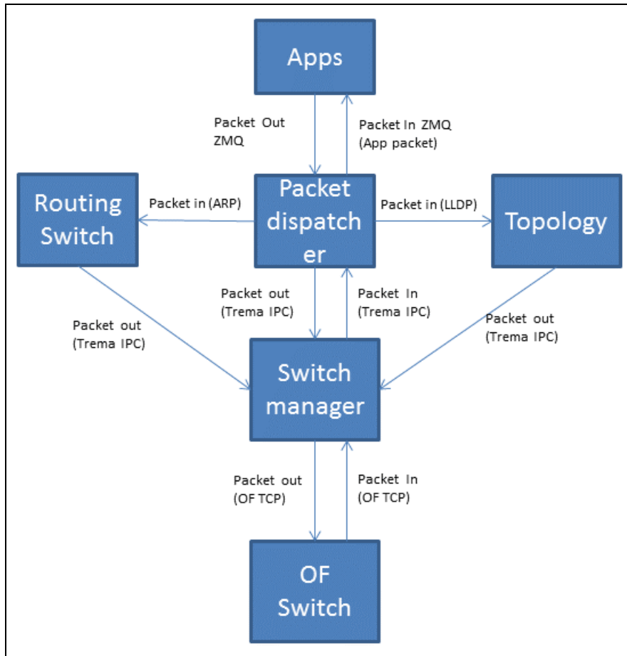
Figure 112 Packet Handling
