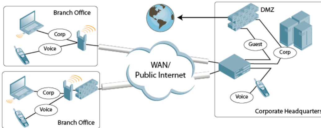
Figure 49 Remote AP with Single Managed device
