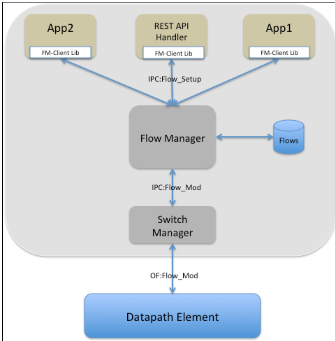
Figure 111 Flow Push
