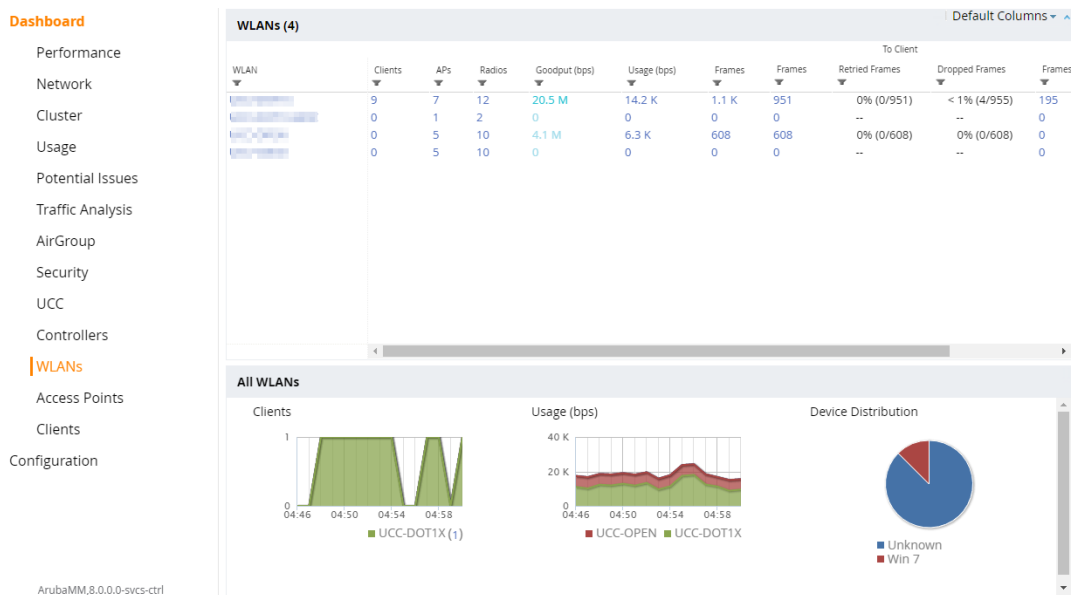
Figure 88 WLANs Page
