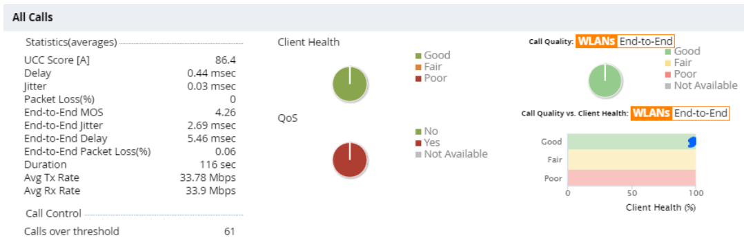
Figure 117 All Calls
