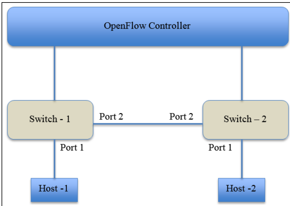
Figure 110 Host Discovery
