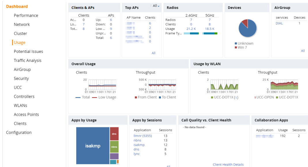
Figure 58 Usage Page
