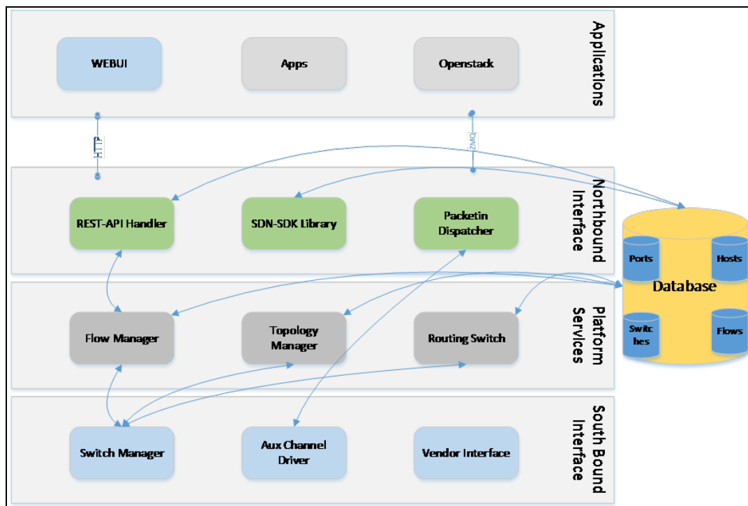
Figure 108 SDN switch Architecture
