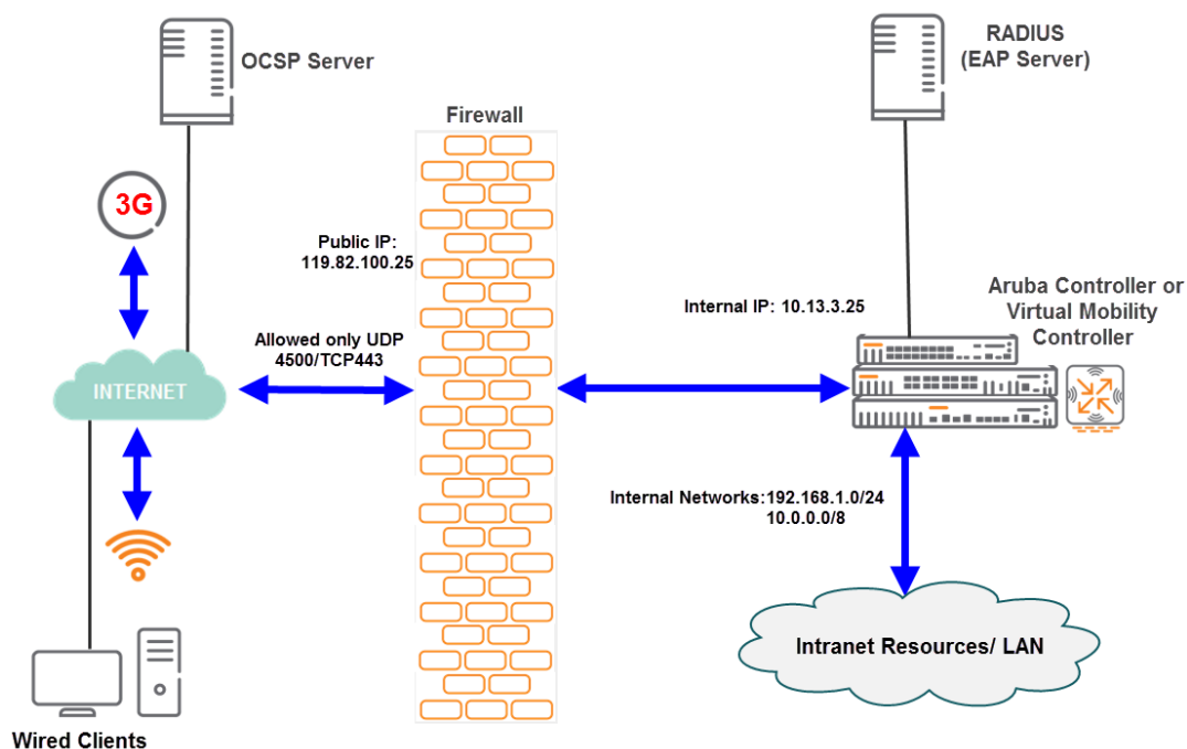
Figure 53 VIA Topology
