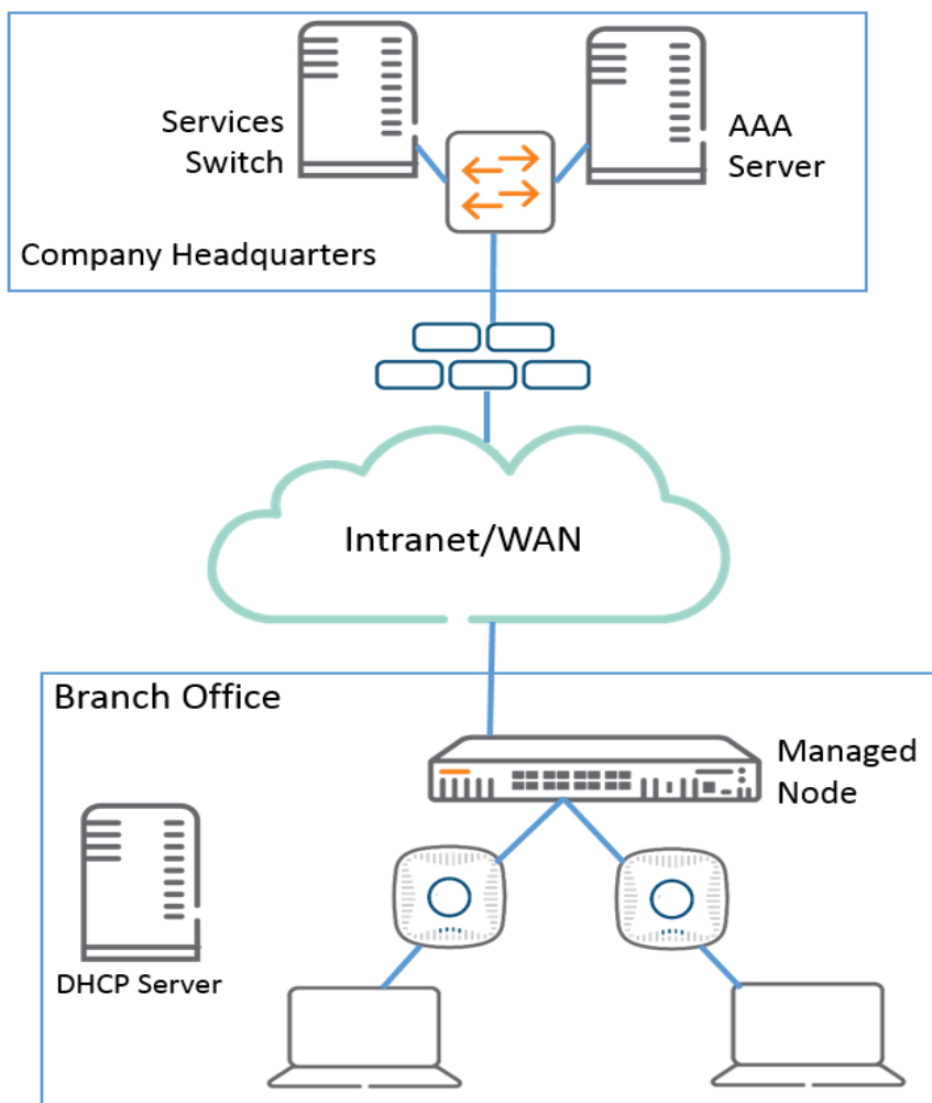
Figure 24 Managed Device Topology
