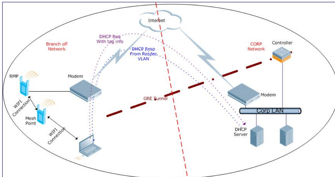
Figure 36 Working of Remote Mesh Portal
