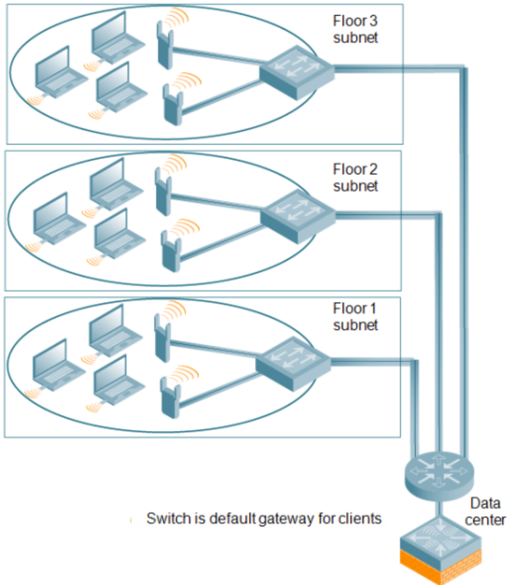
Figure 9 APs All on One Subnet Different from Managed Device Subnets
