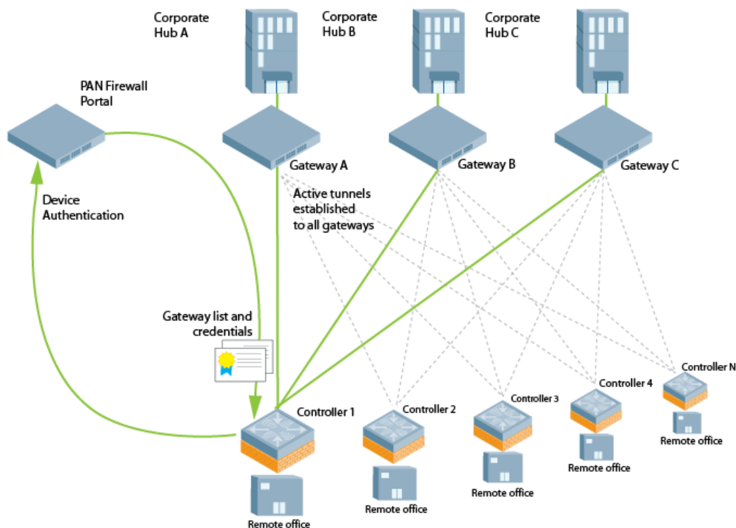
Figure 28 Managed Device and PAN Firewall Integration
