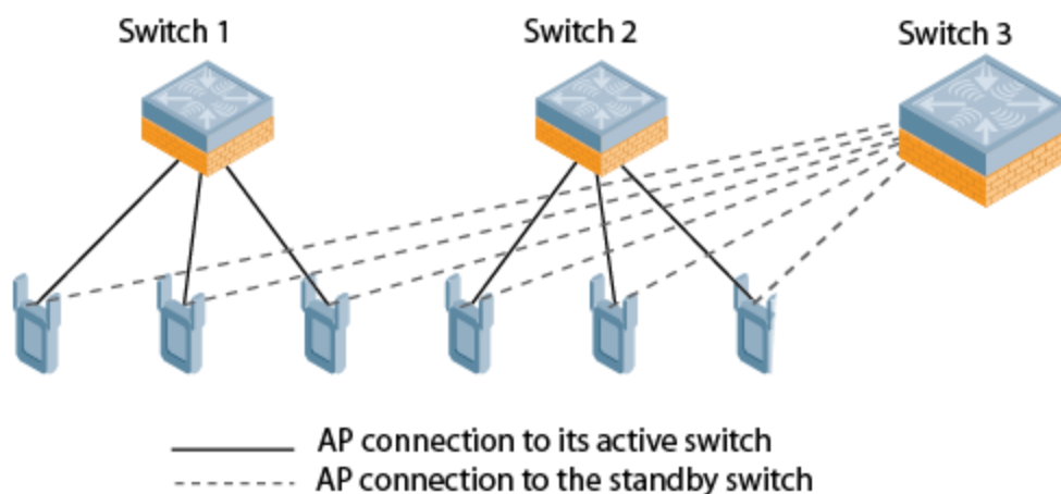
Figure 43 1:1 Active/Standby Deployment
