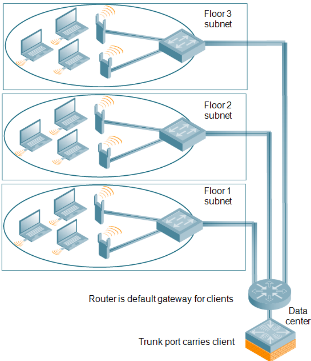
Figure 10 APs on Multiple Different Subnets from Managed Devices
