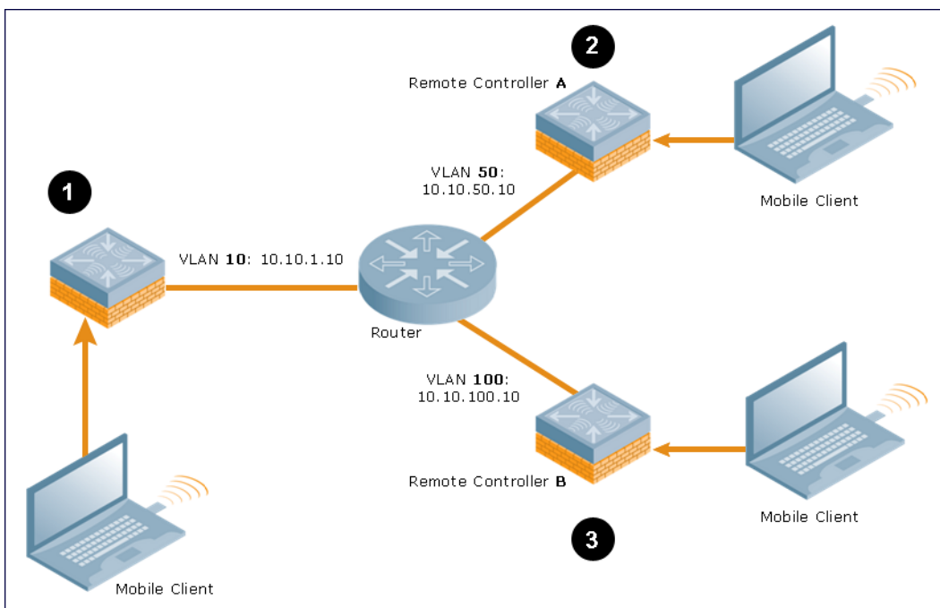
Figure 48 Inter-managed device Mobility
